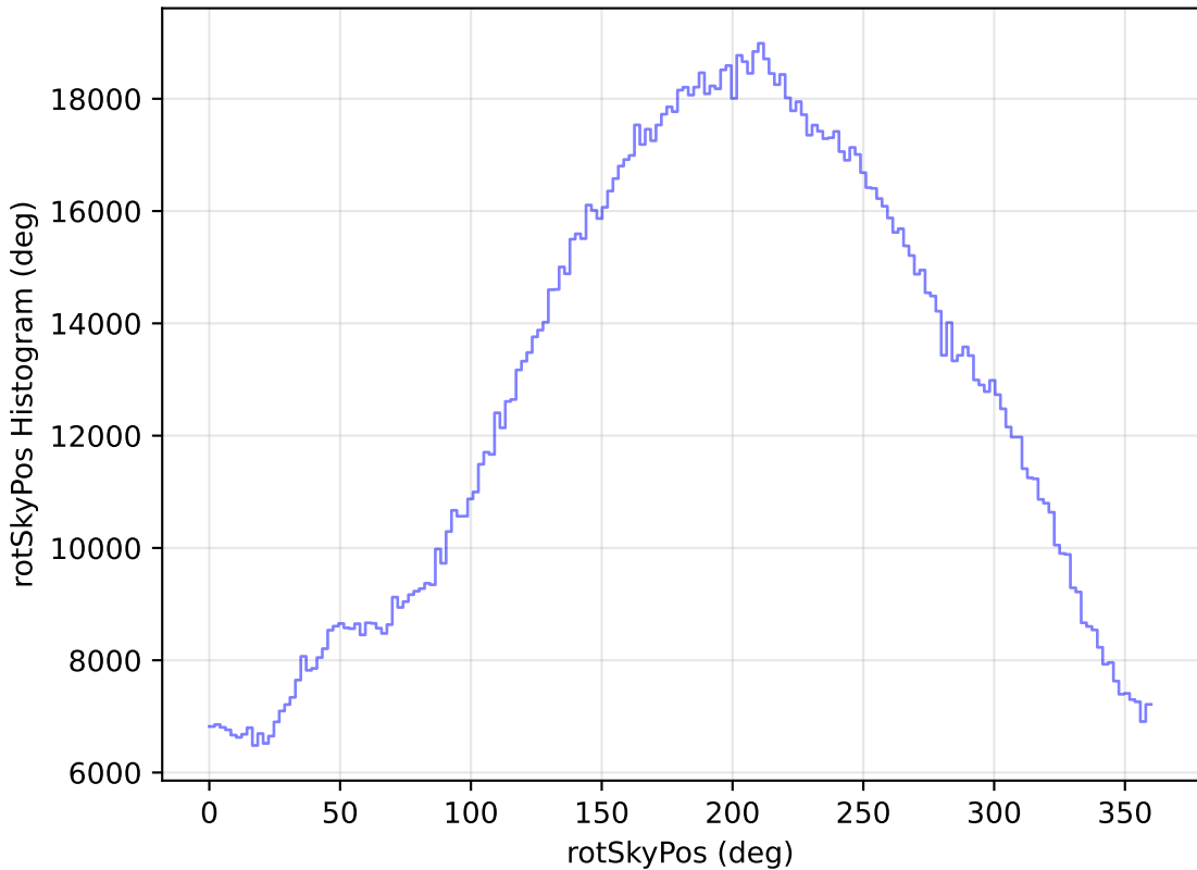
weather_cloudso36v3.4_10yrs All sky all bands: rotSkyPos Histogram
