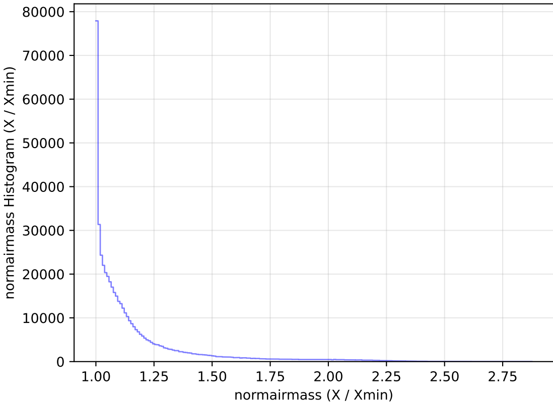
weather_cloudso36v3.4_10yrs WFD r band: normairmass Histogram
