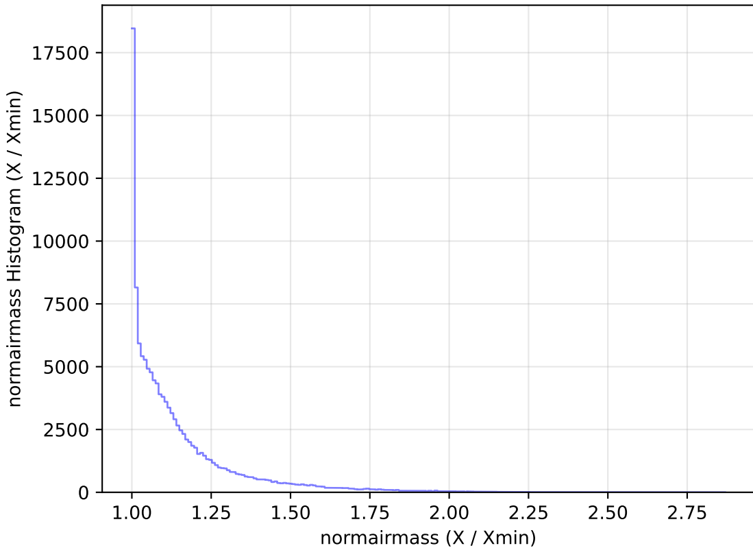
weather_cloudso36v3.4_10yrs All sky u band: normairmass Histogram
