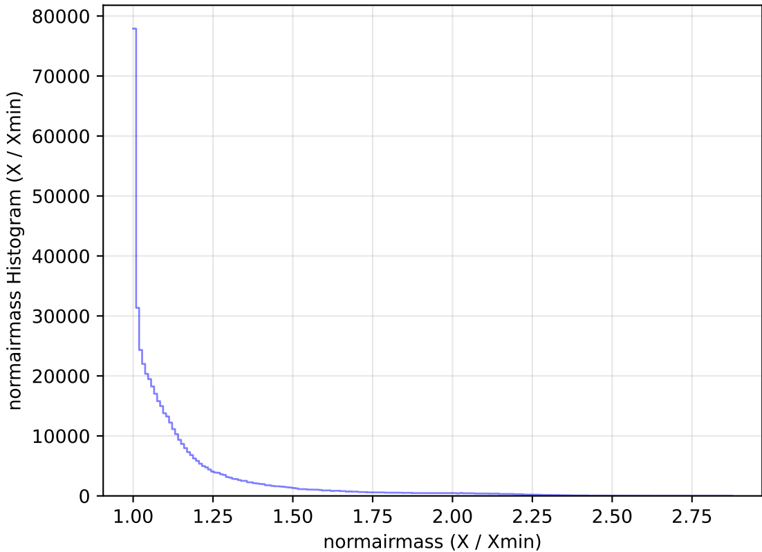
weather_cloudso36v3.4_10yrs All sky r band: normairmass Histogram
