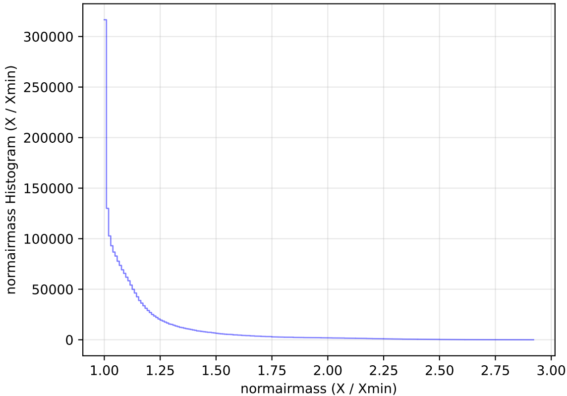
weather_cloudso36v3.4_10yrs All sky all bands: normairmass Histogram
