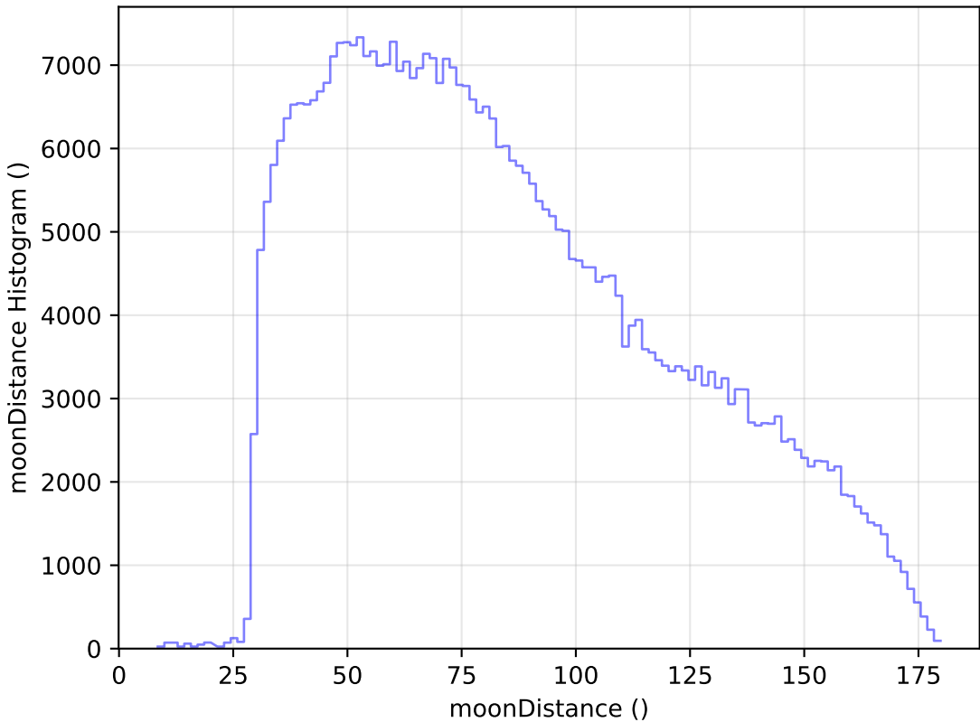
weather_cloudso36v3.4_10yrs WFD z band: moonDistance Histogram
