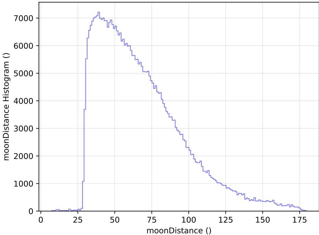
weather_cloudso36v3.4_10yrs WFD y band: moonDistance Histogram
