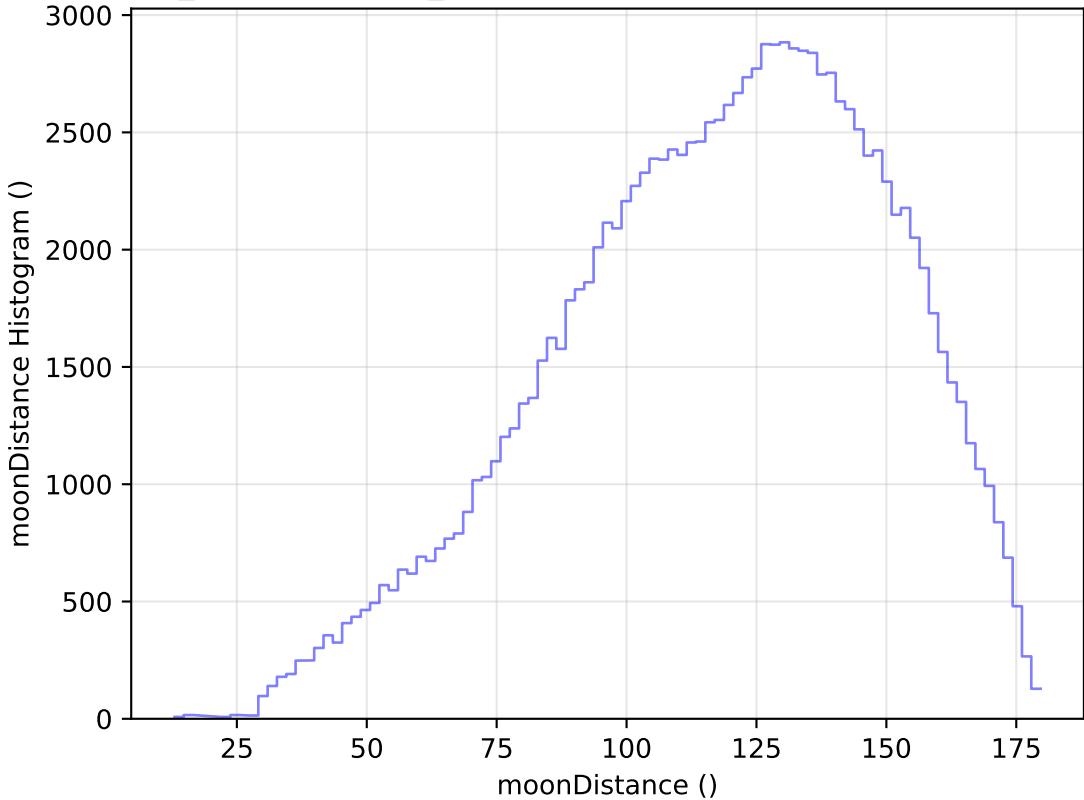
weather_cloudso36v3.4_10yrs WFD u band: moonDistance Histogram
