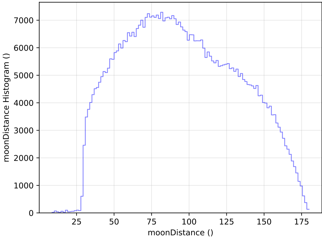
weather_cloudso36v3.4_10yrs WFD i band: moonDistance Histogram
