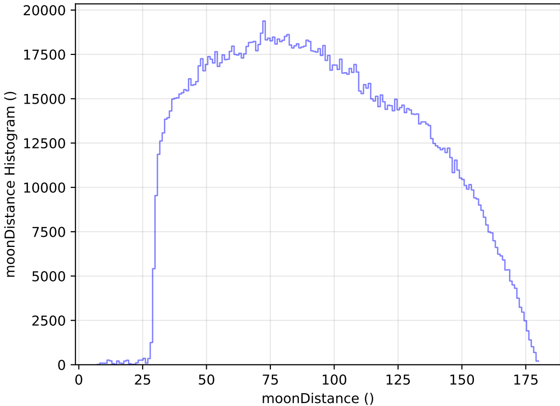
weather_cloudso36v3.4_10yrs WFD all bands: moonDistance Histogram
