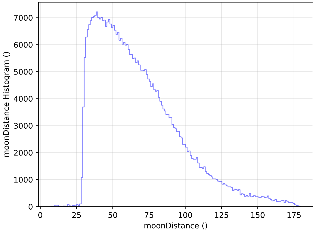
weather_cloudso36v3.4_10yrs All sky y band: moonDistance Histogram
