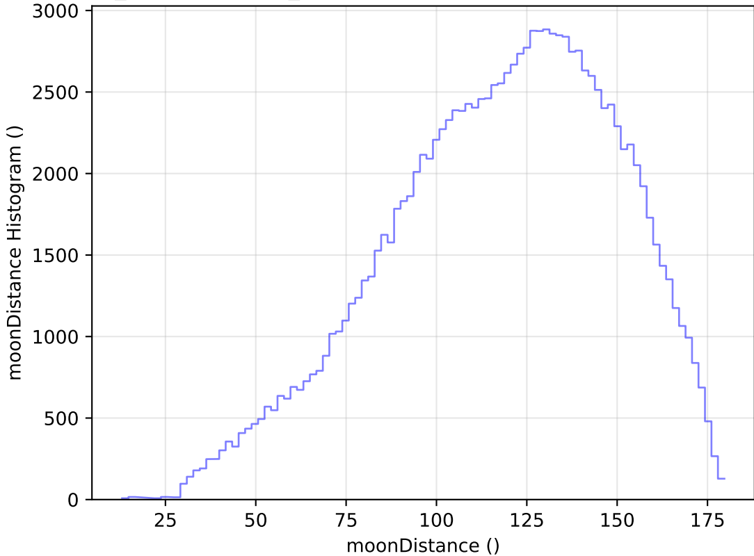
weather_cloudso36v3.4_10yrs All sky u band: moonDistance Histogram
