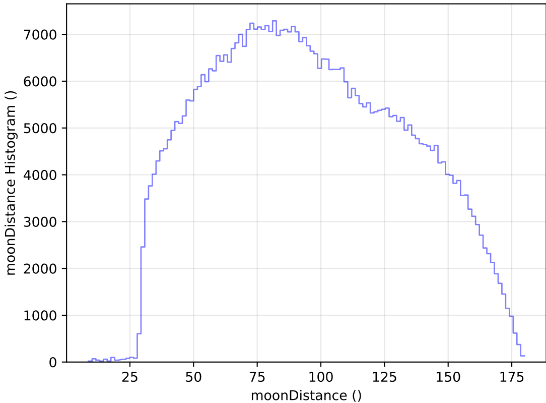
weather_cloudso36v3.4_10yrs All sky i band: moonDistance Histogram
