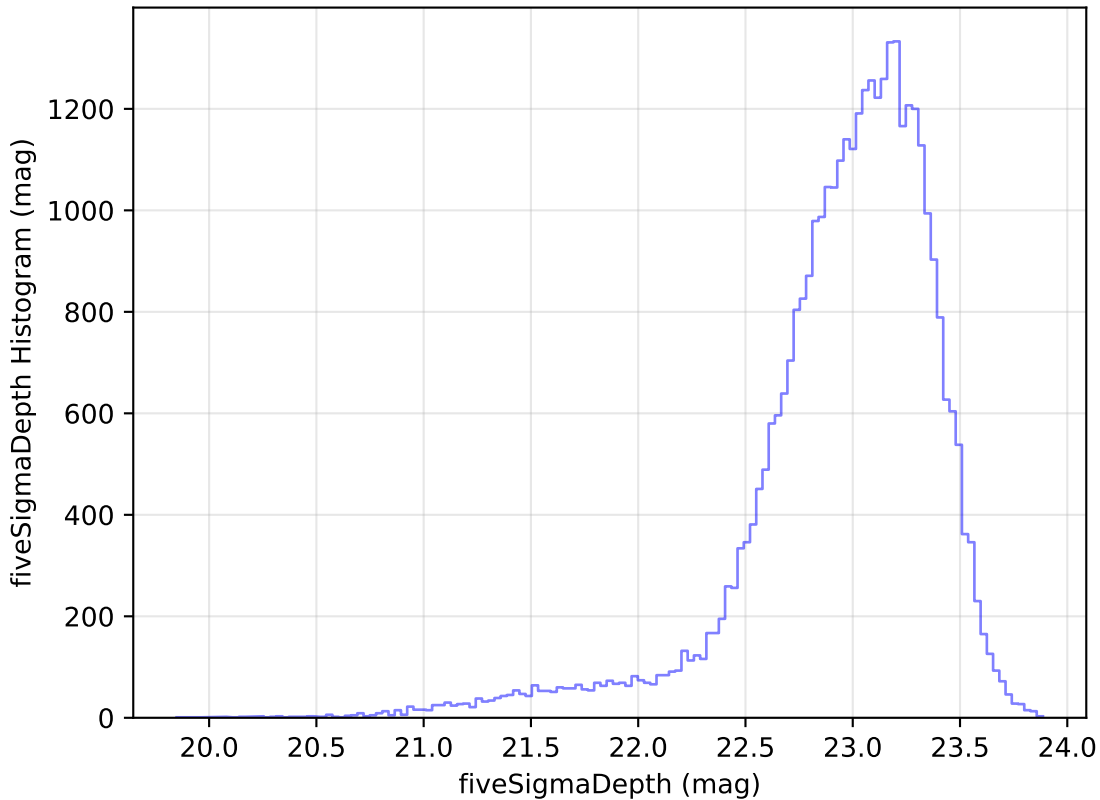
weather_cloudso36v3.4_10yrs Yr 1 z band: fiveSigmaDepth Histogram
