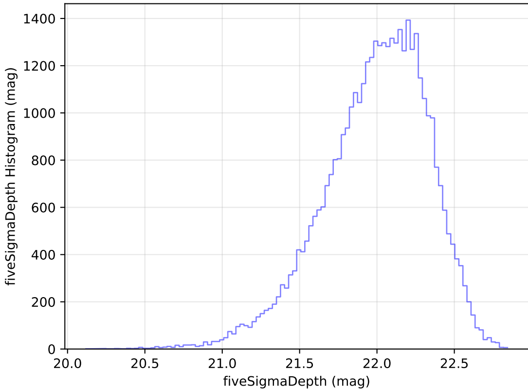
weather_cloudso36v3.4_10yrs Yr 1 y band: fiveSigmaDepth Histogram
