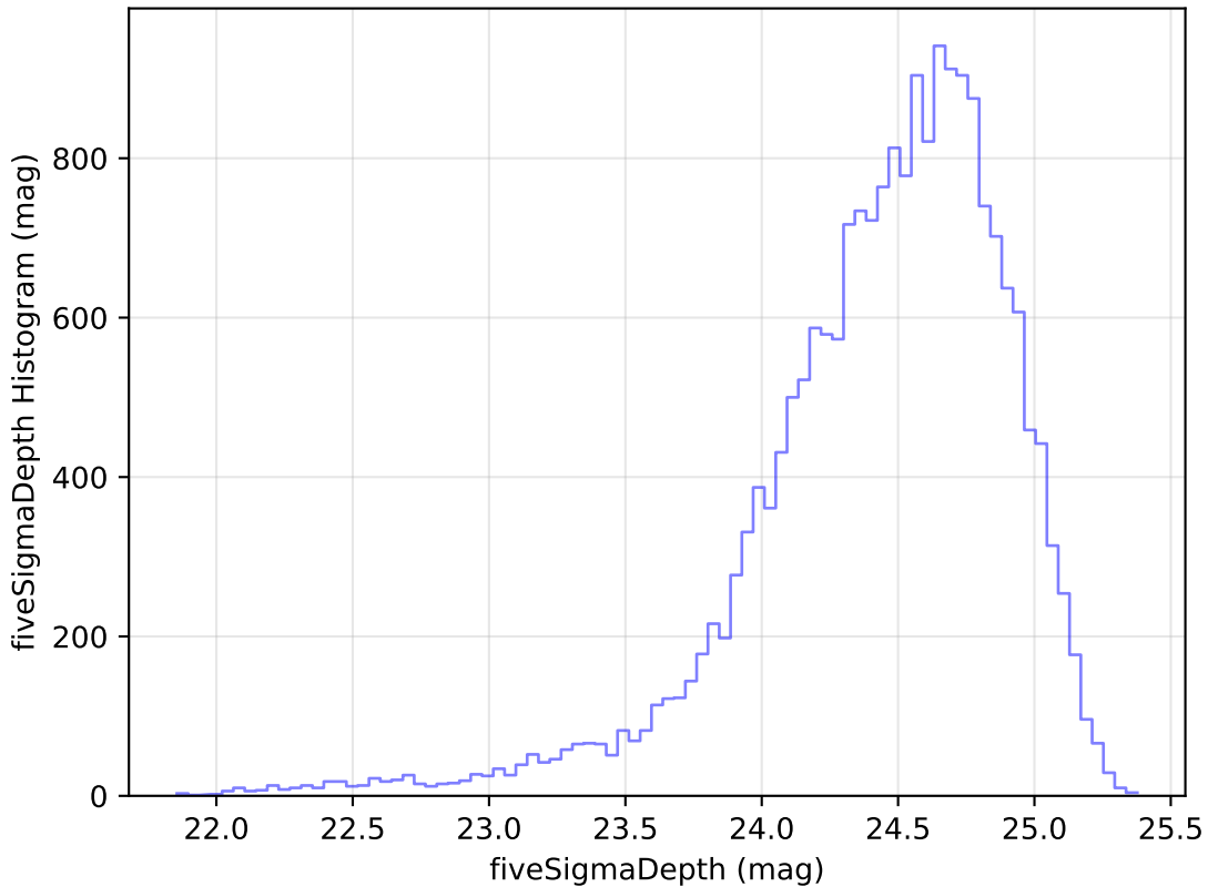
weather_cloudso36v3.4_10yrs Yr 1 g band: fiveSigmaDepth Histogram
