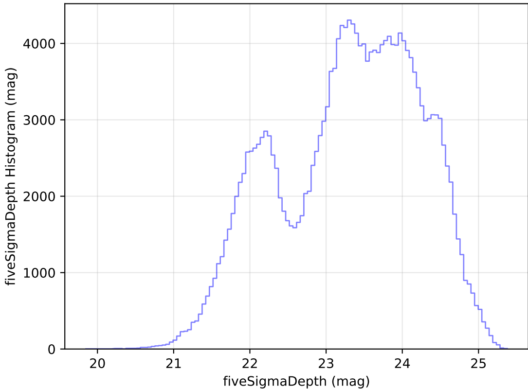
weather_cloudso36v3.4_10yrs Yr 1 all bands: fiveSigmaDepth Histogram
