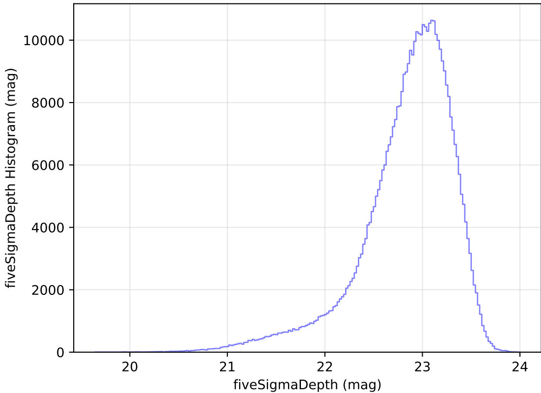
weather_cloudso36v3.4_10yrs WFD z band: fiveSigmaDepth Histogram
