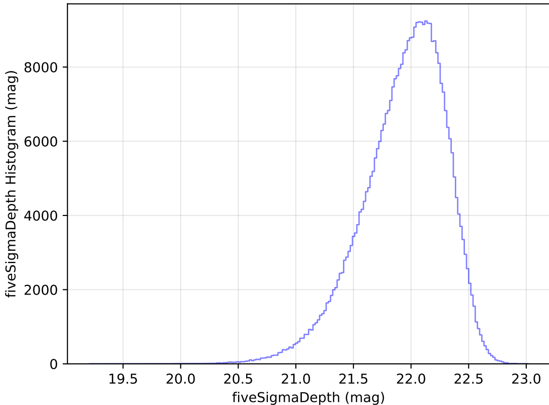
weather_cloudso36v3.4_10yrs WFD y band: fiveSigmaDepth Histogram
