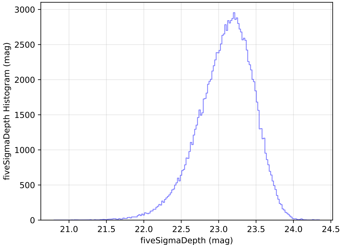
weather_cloudso36v3.4_10yrs WFD u band: fiveSigmaDepth Histogram
