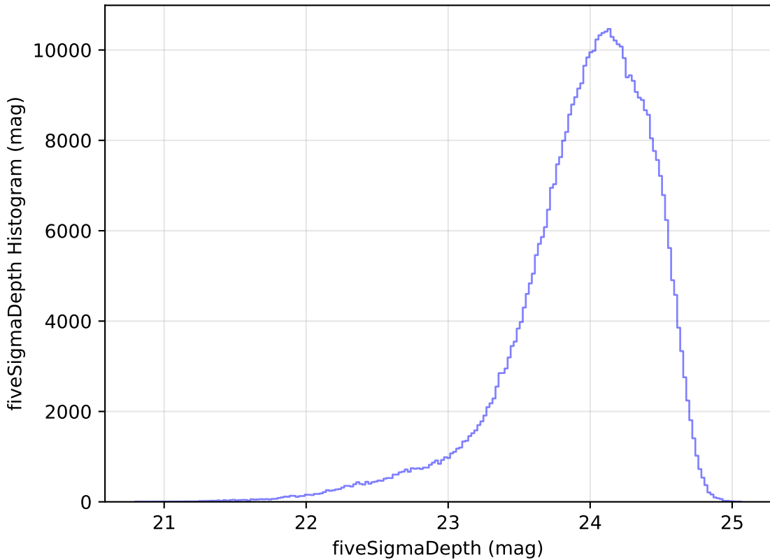
weather_cloudso36v3.4_10yrs WFD r band: fiveSigmaDepth Histogram
