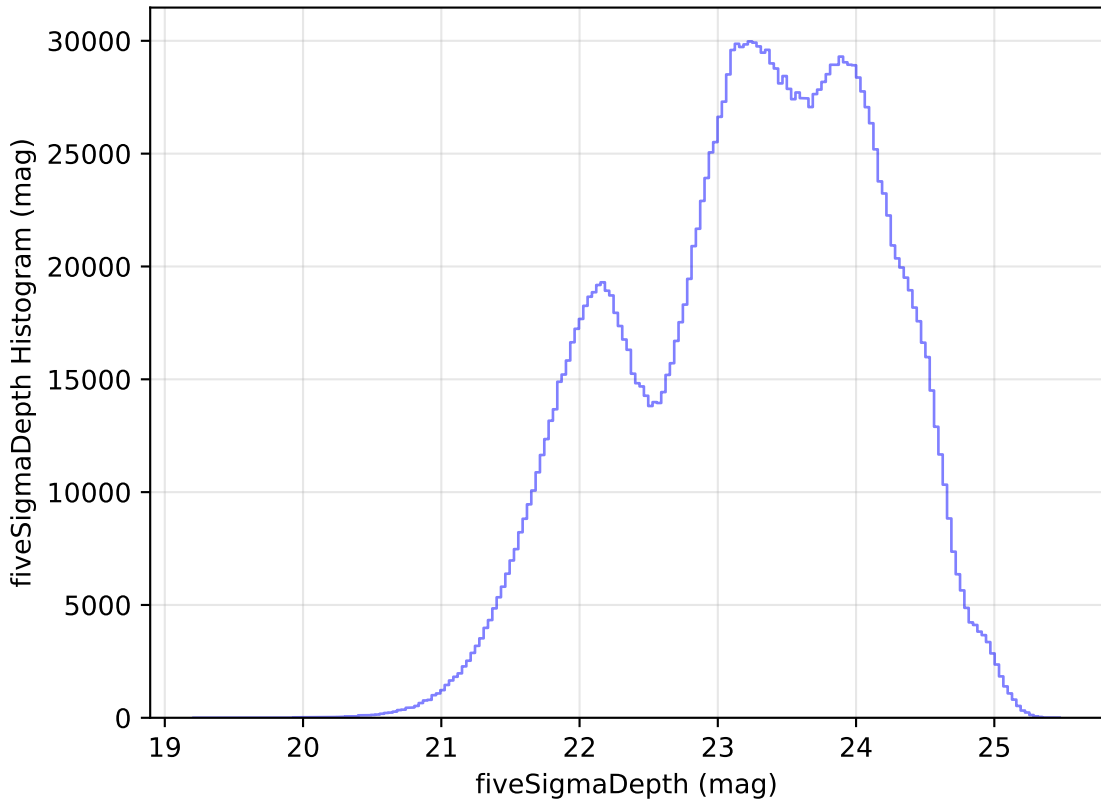
weather_cloudso36v3.4_10yrs WFD all bands: fiveSigmaDepth Histogram
