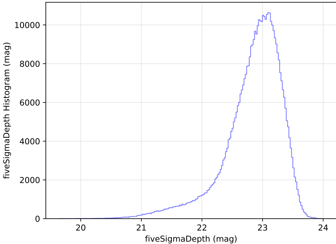
weather_cloudso36v3.4_10yrs All sky z band: fiveSigmaDepth Histogram
