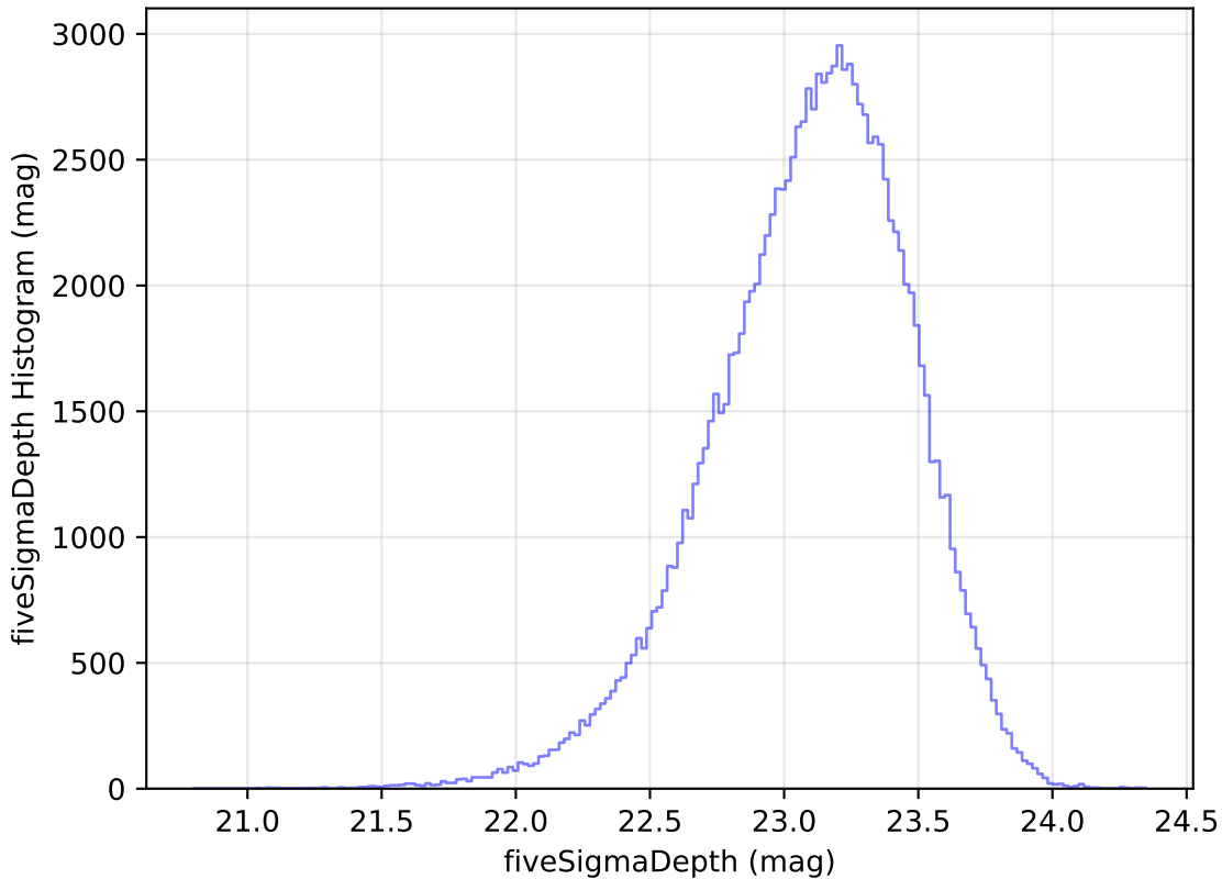
weather_cloudso36v3.4_10yrs All sky u band: fiveSigmaDepth Histogram
