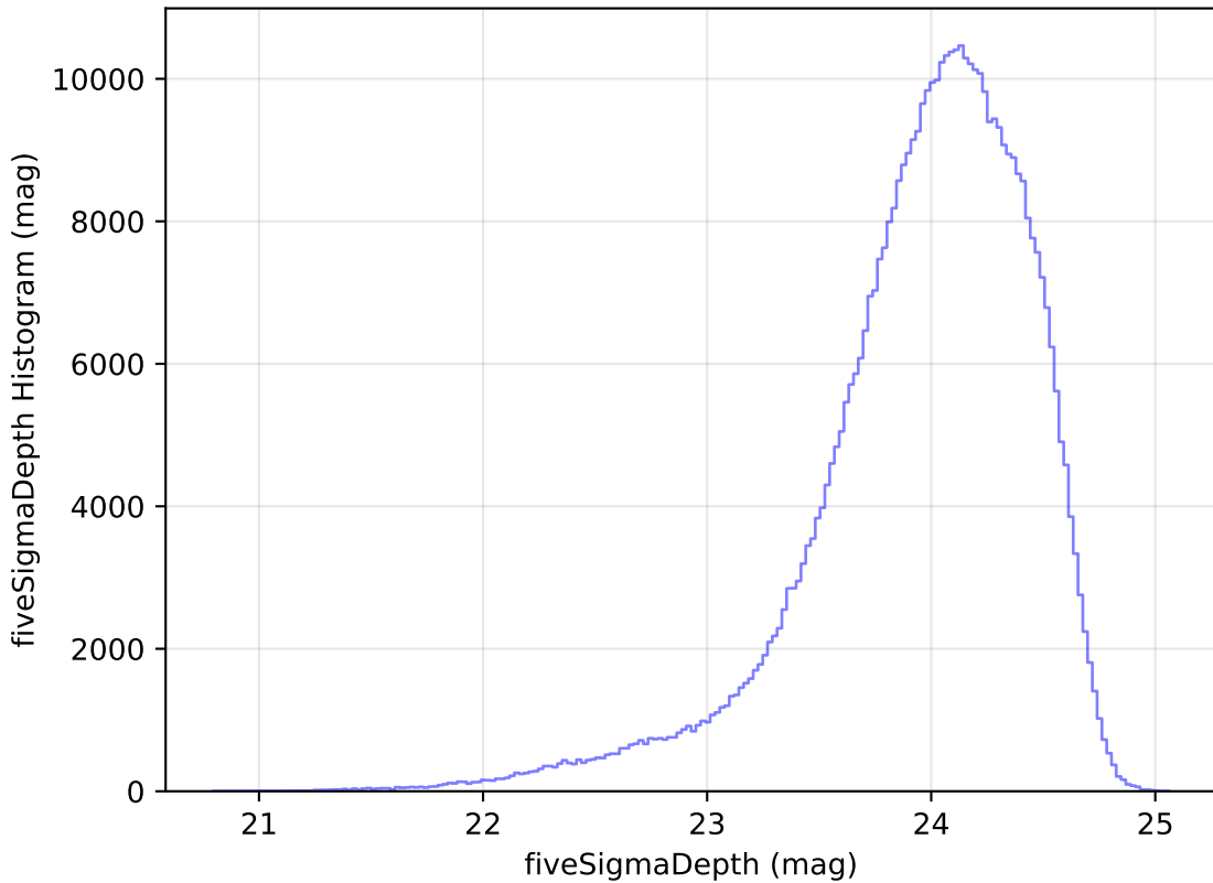
weather_cloudso36v3.4_10yrs All sky r band: fiveSigmaDepth Histogram
