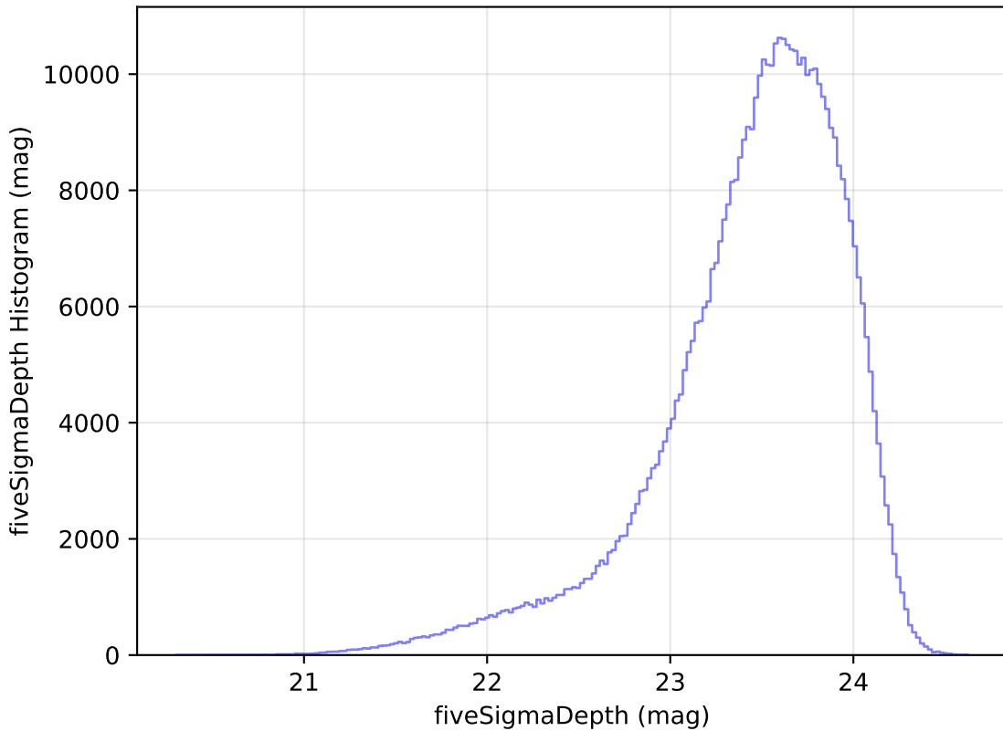
weather_cloudso36v3.4_10yrs All sky i band: fiveSigmaDepth Histogram
