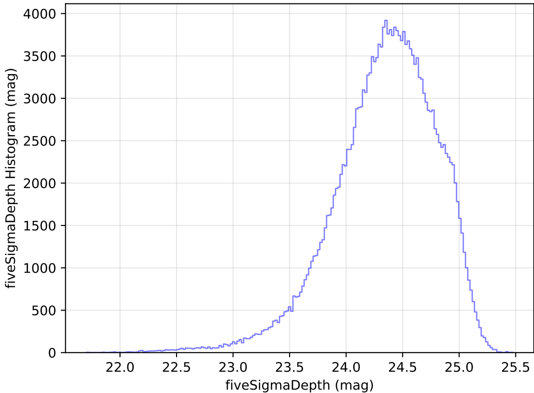
weather_cloudso36v3.4_10yrs All sky g band: fiveSigmaDepth Histogram
