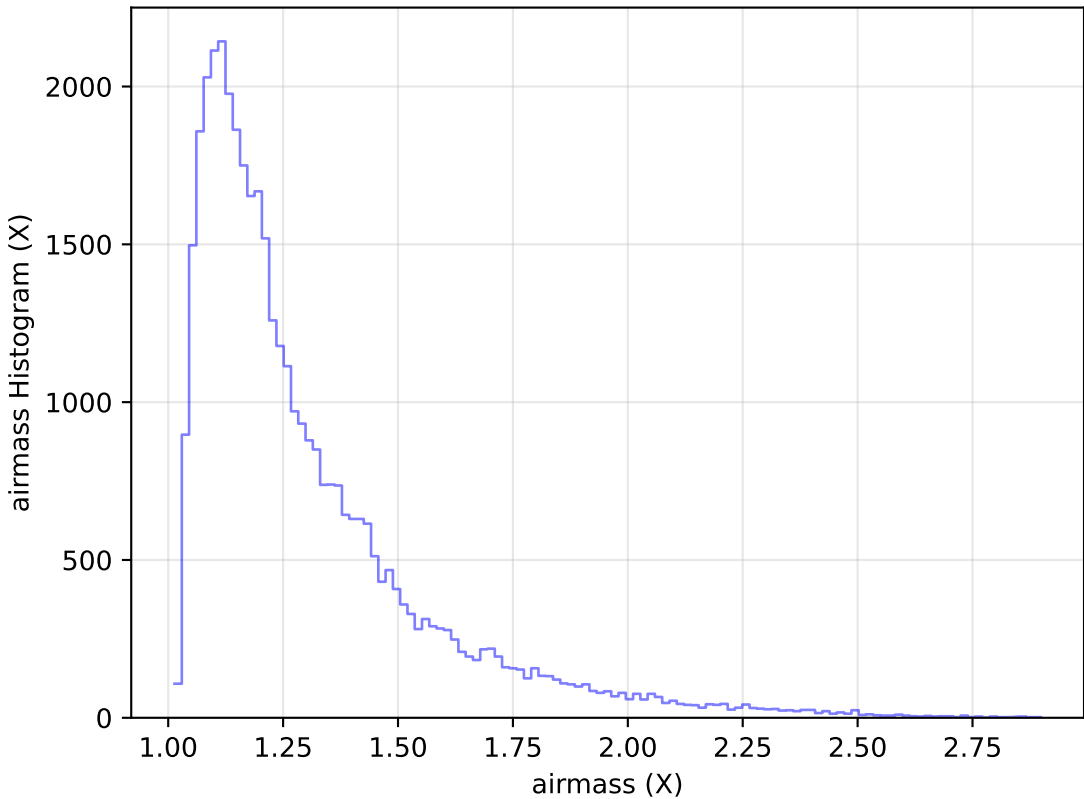
weather_cloudso36v3.4_10yrs Yr 1 y band: airmass Histogram
