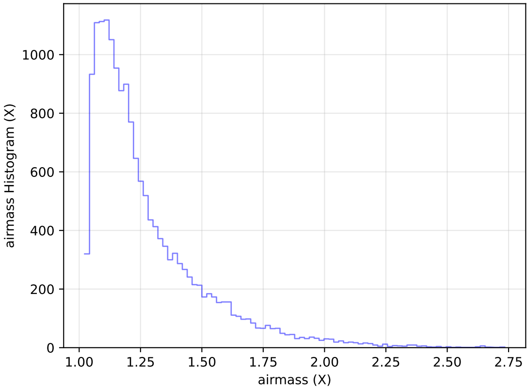
weather_cloudso36v3.4_10yrs Yr 1 u band: airmass Histogram
