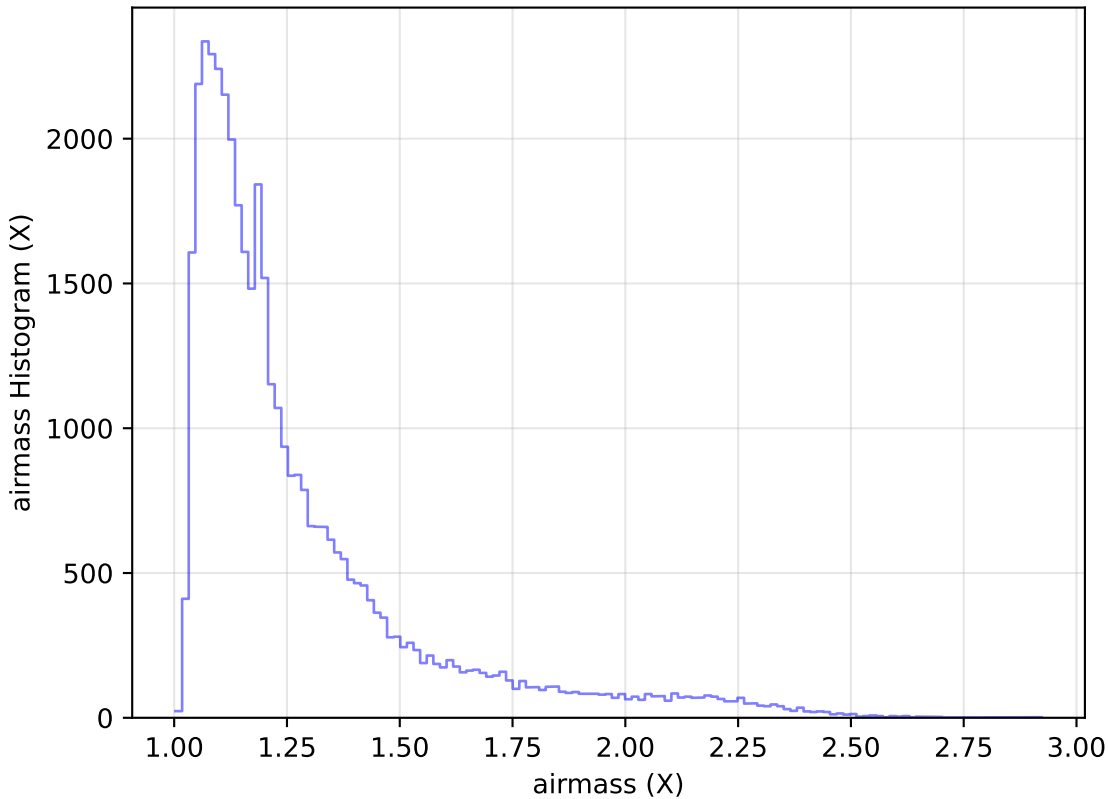
weather_cloudso36v3.4_10yrs Yr 1 r band: airmass Histogram
