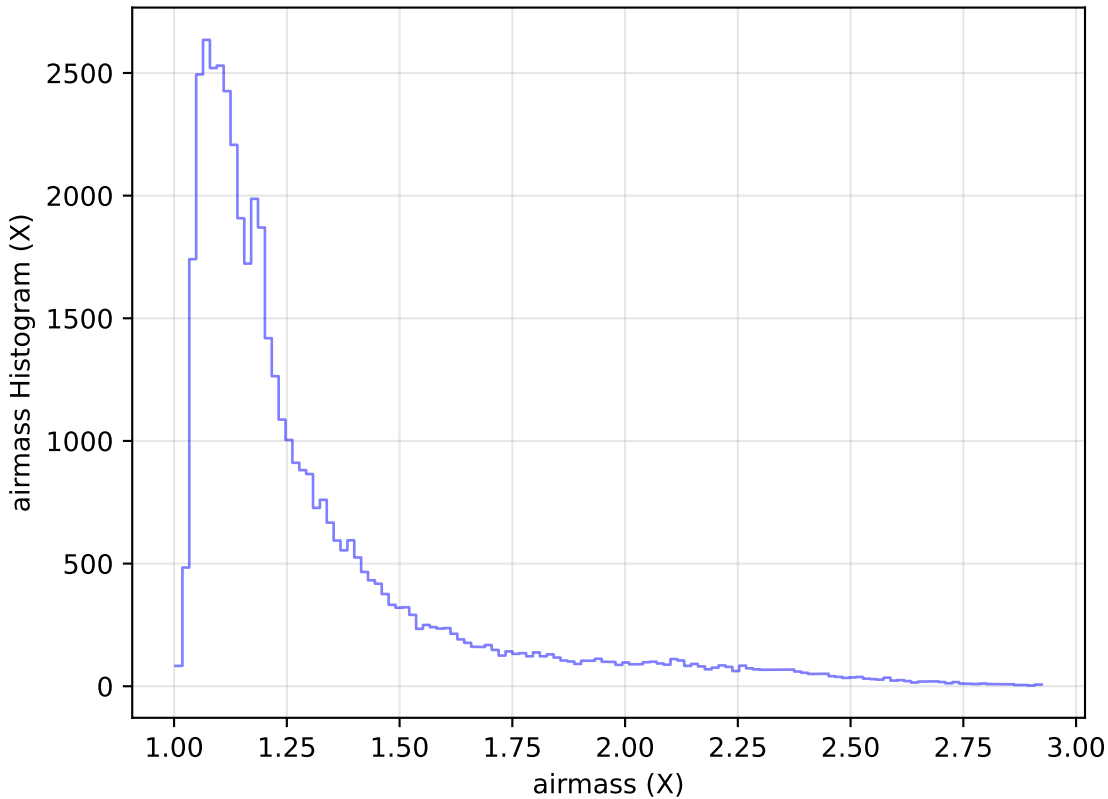
weather_cloudso36v3.4_10yrs Yr 1 i band: airmass Histogram
