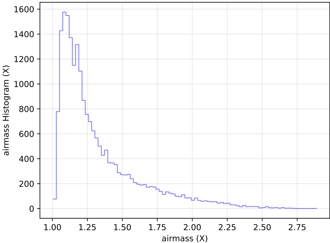
weather_cloudso36v3.4_10yrs Yr 1 g band: airmass Histogram
