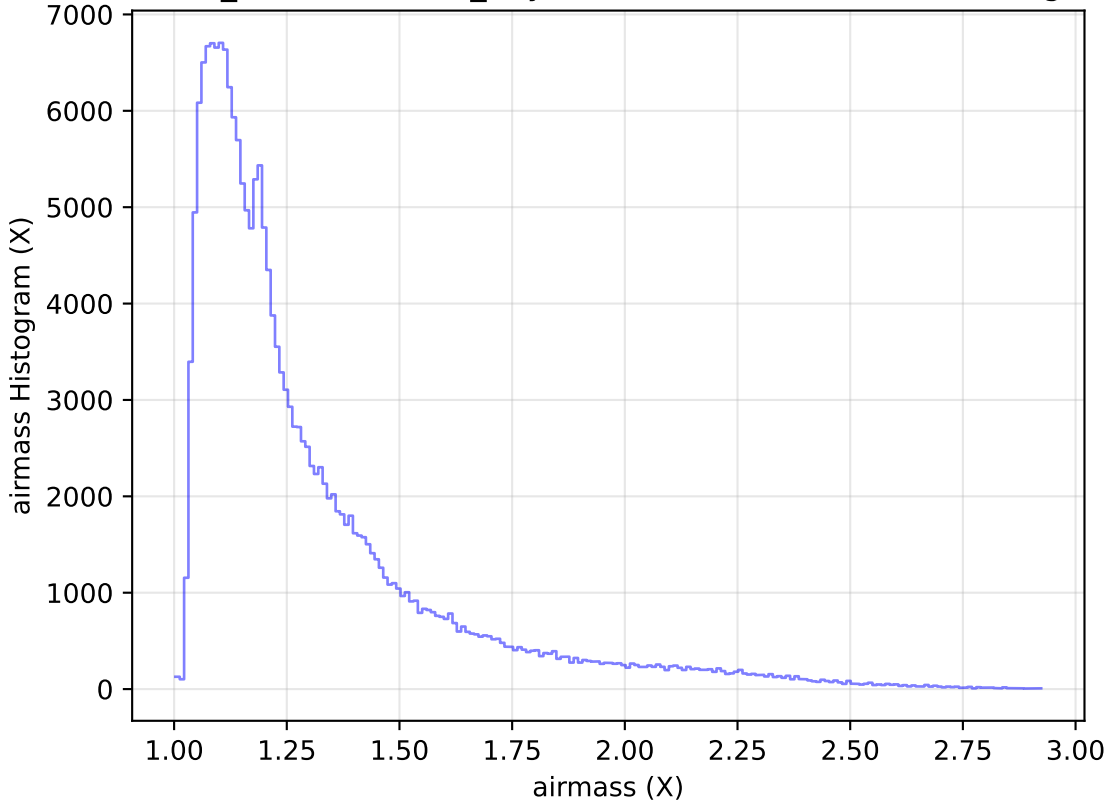
weather_cloudso36v3.4_10yrs Yr 1 all bands: airmass Histogram
