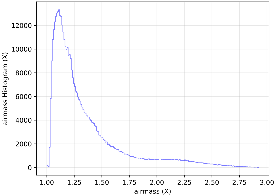
weather_cloudso36v3.4_10yrs WFD z band: airmass Histogram
