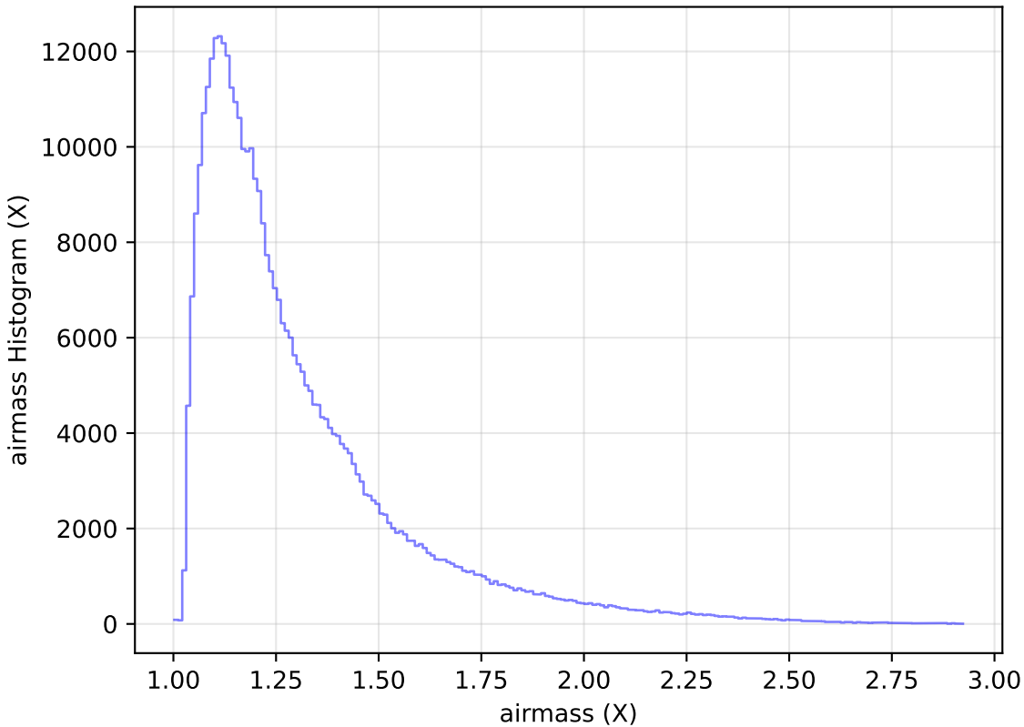
weather_cloudso36v3.4_10yrs WFD y band: airmass Histogram
