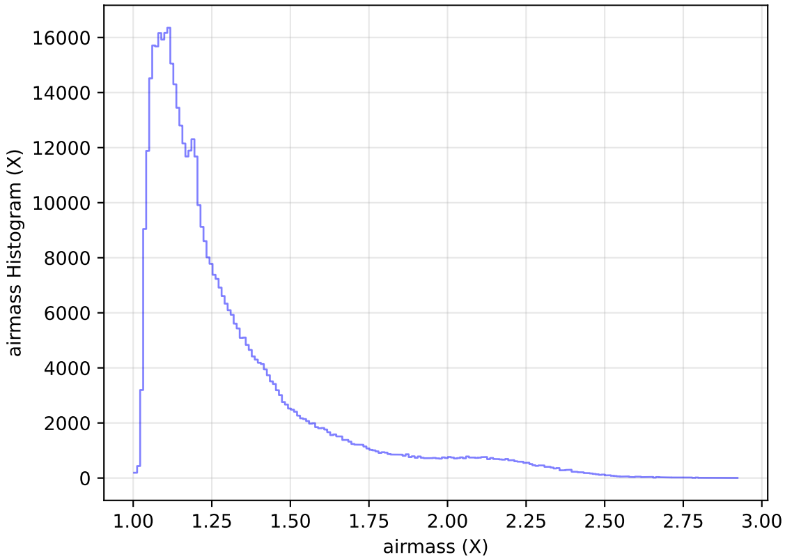
weather_cloudso36v3.4_10yrs WFD r band: airmass Histogram
