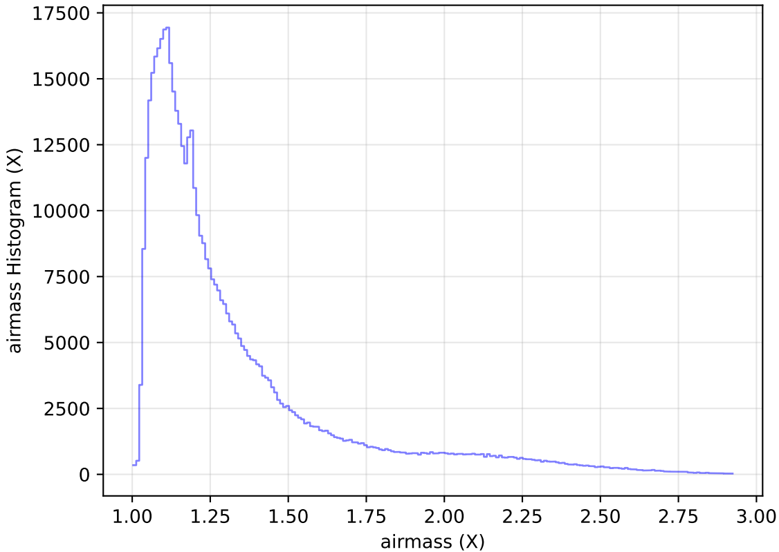
weather_cloudso36v3.4_10yrs WFD i band: airmass Histogram
