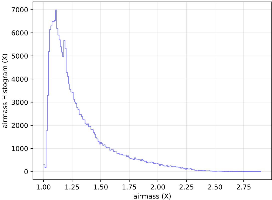
weather_cloudso36v3.4_10yrs WFD g band: airmass Histogram
