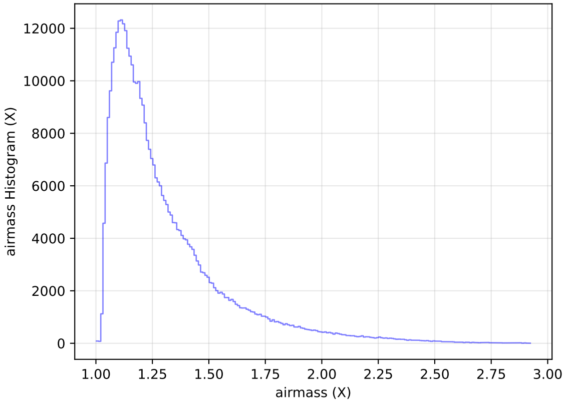
weather_cloudso36v3.4_10yrs All sky y band: airmass Histogram
