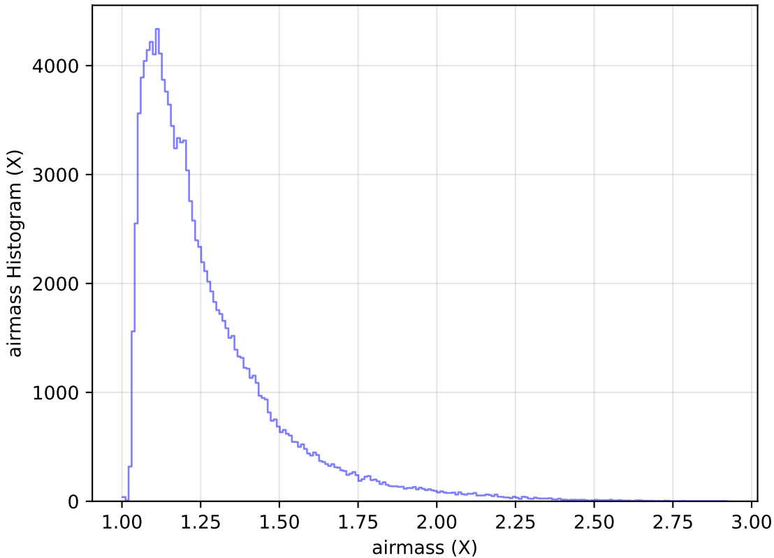
weather_cloudso36v3.4_10yrs All sky u band: airmass Histogram
