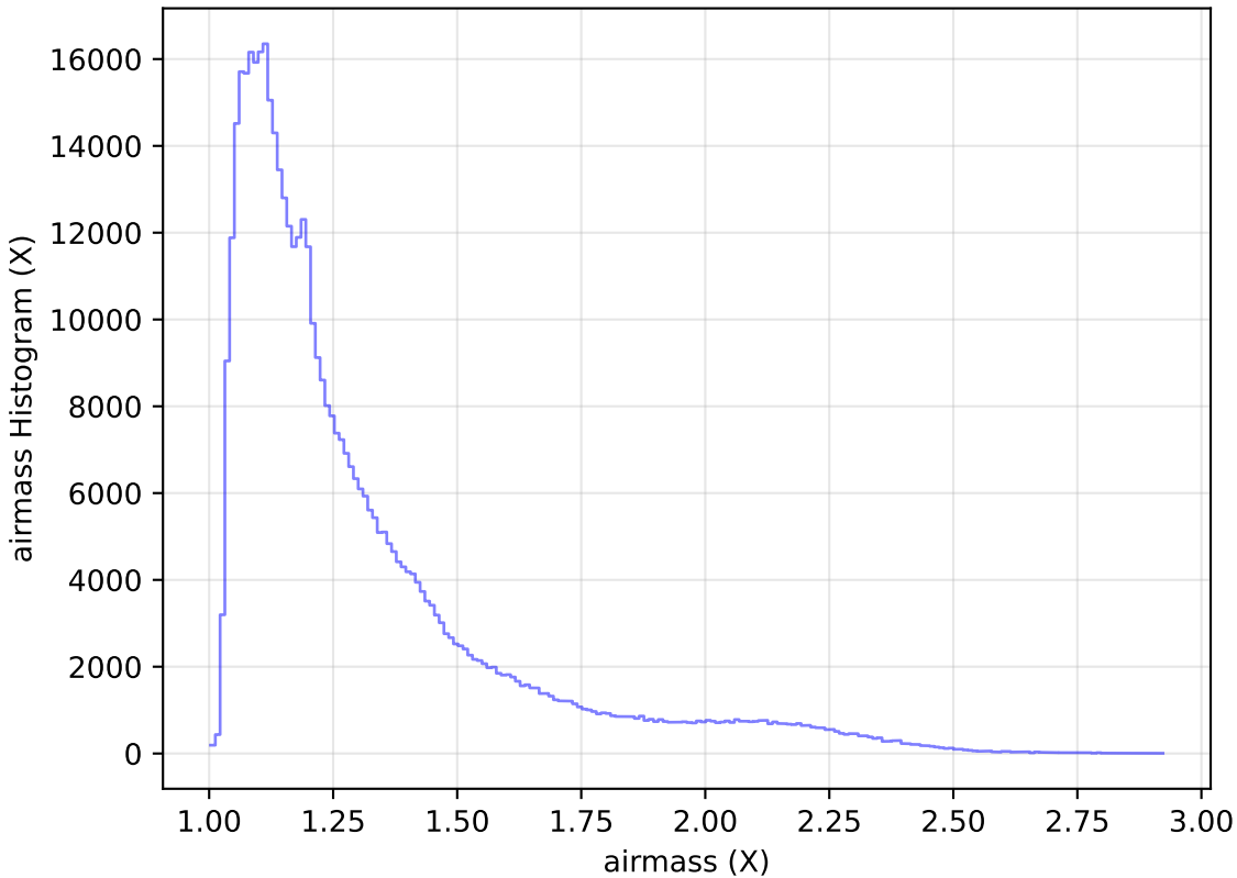
weather_cloudso36v3.4_10yrs All sky r band: airmass Histogram
