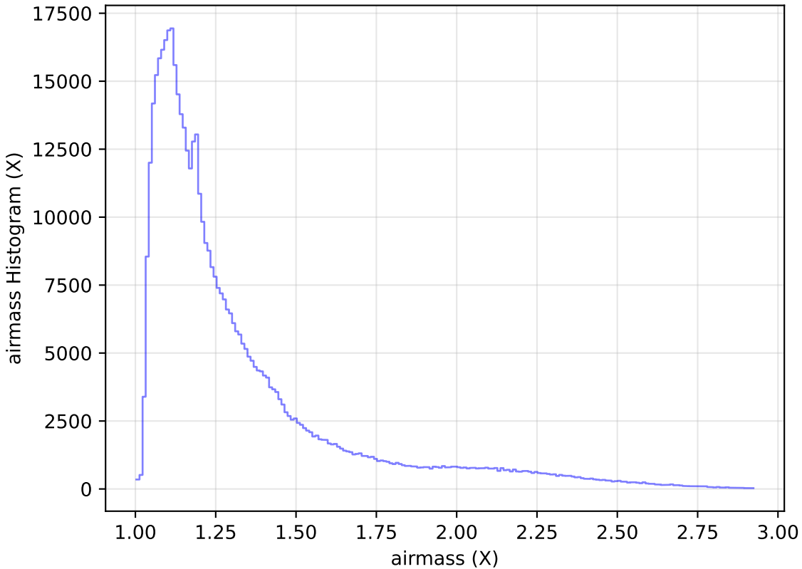
weather_cloudso36v3.4_10yrs All sky i band: airmass Histogram
