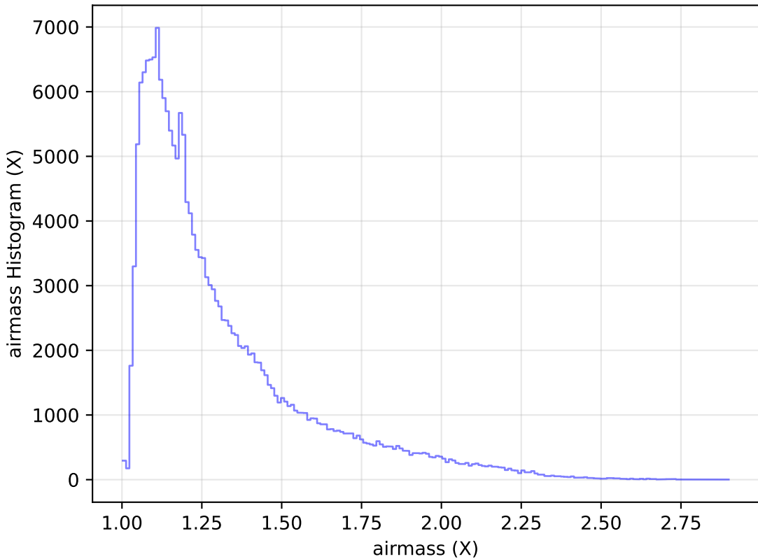
weather_cloudso36v3.4_10yrs All sky g band: airmass Histogram
