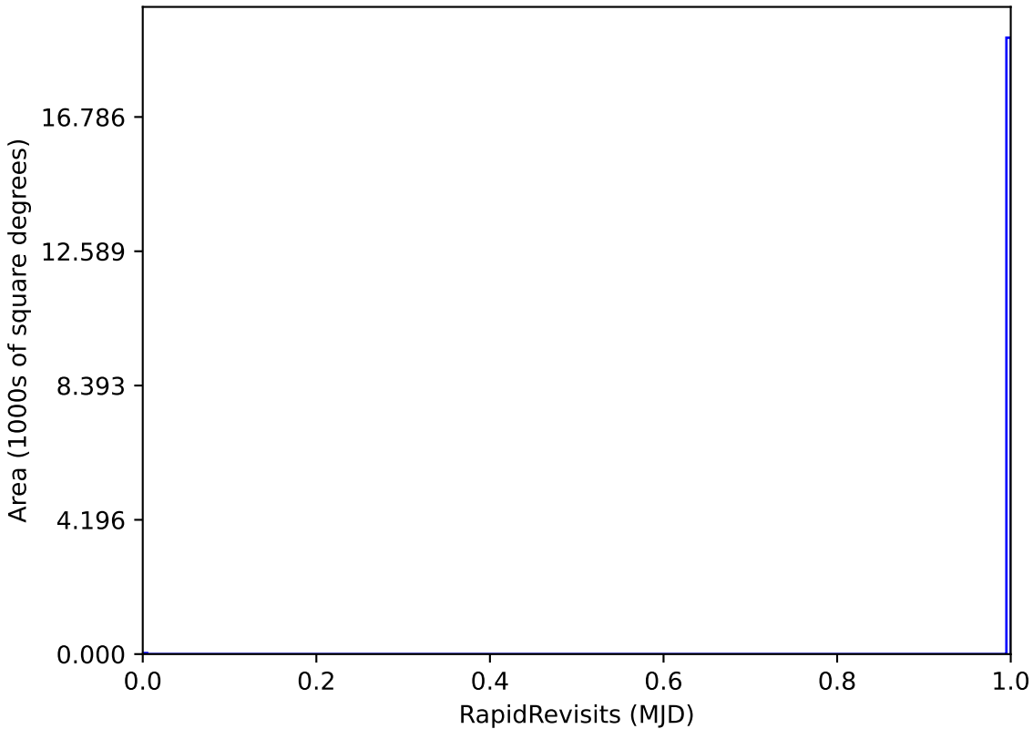
weather_cloudso36v3.4_10yrs WFD: RapidRevisits
