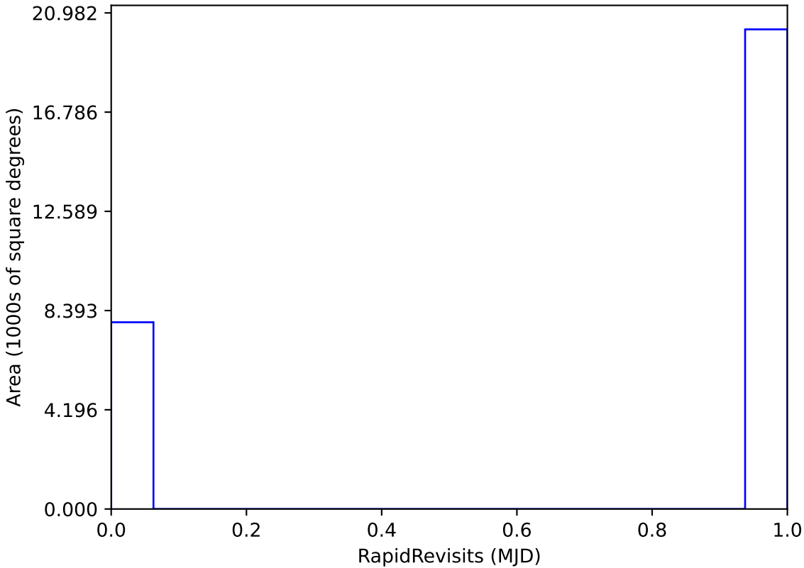
weather_cloudso36v3.4_10yrs All sky: RapidRevisits
