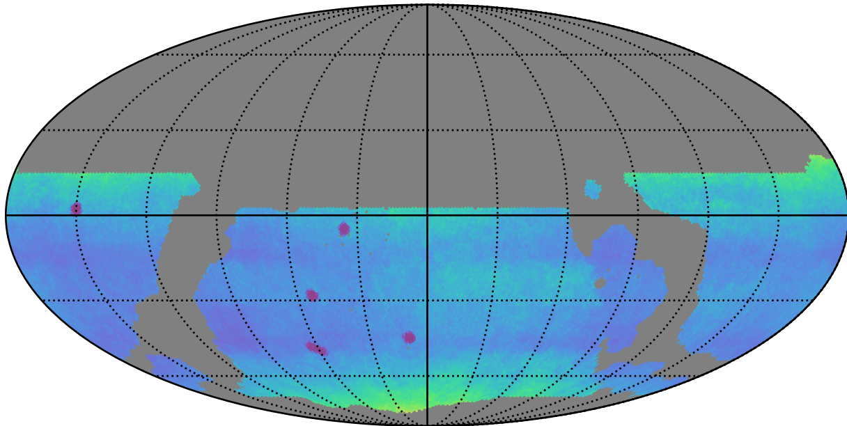
weather_cloudso36v3.4_10yrs WFD: Proper Motion Uncert @ 24.0
