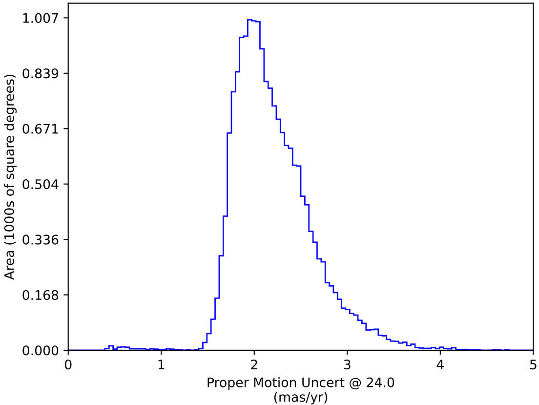
weather_cloudso36v3.4_10yrs WFD: Proper Motion Uncert @ 24.0
