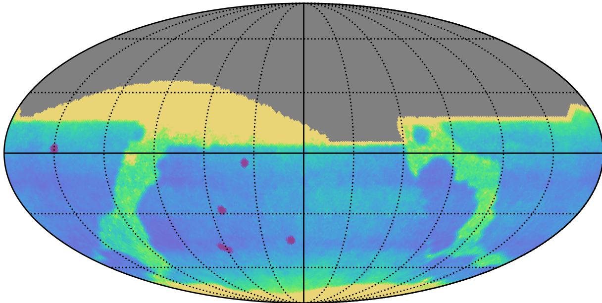
weather_cloudso36v3.4_10yrs All sky: Proper Motion Uncert @ 24.0
