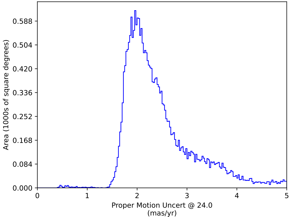
weather_cloudso36v3.4_10yrs All sky: Proper Motion Uncert @ 24.0
