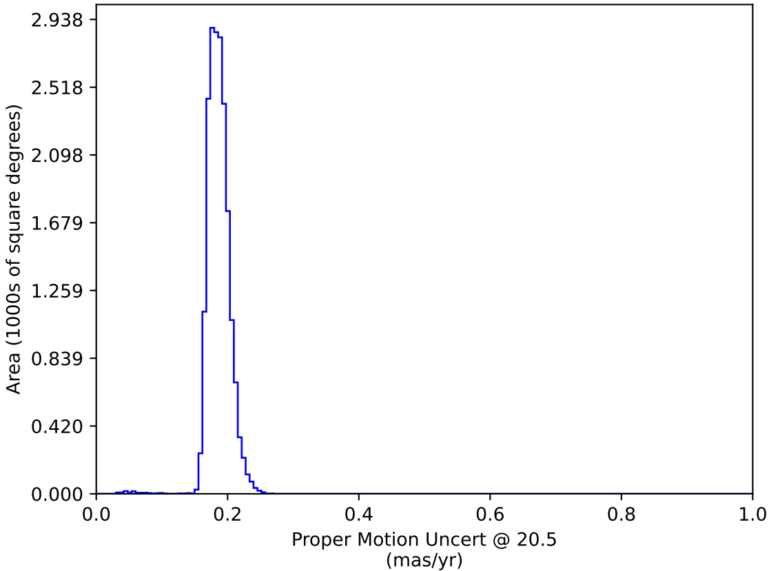
weather_cloudso36v3.4_10yrs WFD: Proper Motion Uncert @ 20.5
